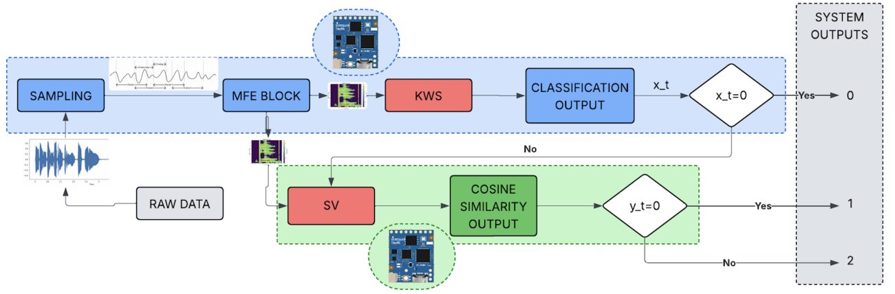
Figure 4.1: Software Pipeline
