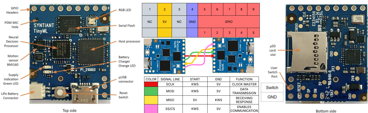
Figure 4.4: System Hardware Setup
