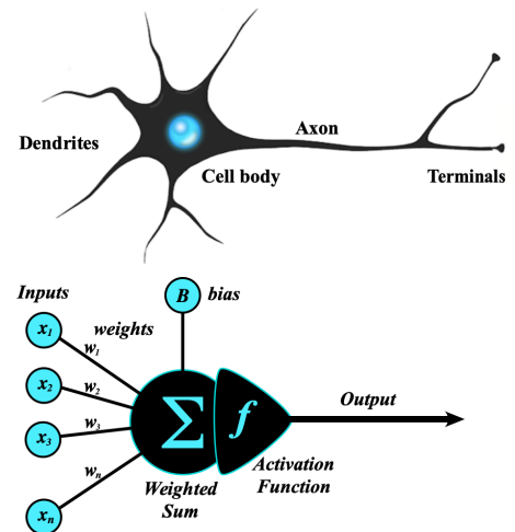
Figure 2.4: Neuron structure [31]
