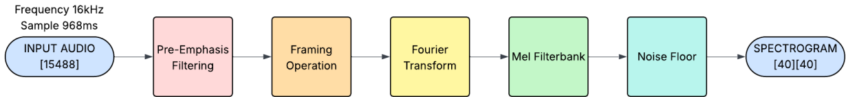
Figure 2.3: Syntiant Audio Block Processing
